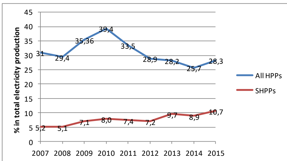
Figure 1. Share (in %) of all HPPs including small HPPs (upper curve) and share (in %) of small HPPs in total annual electricity generation from 2007 to 2015.
